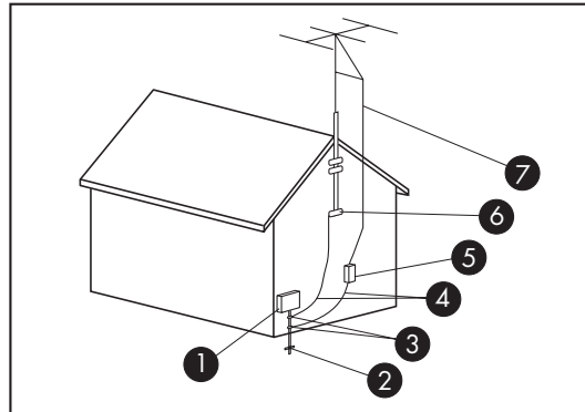
Antenna Grounding
